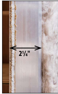
A DRV EXCLUSIVE Thicker side walls allow for high density wool insulation, with an integrated 1/4" thick foam core moisture barrier , to eliminate condensation and add an additional insulating moisture barrier layer.
